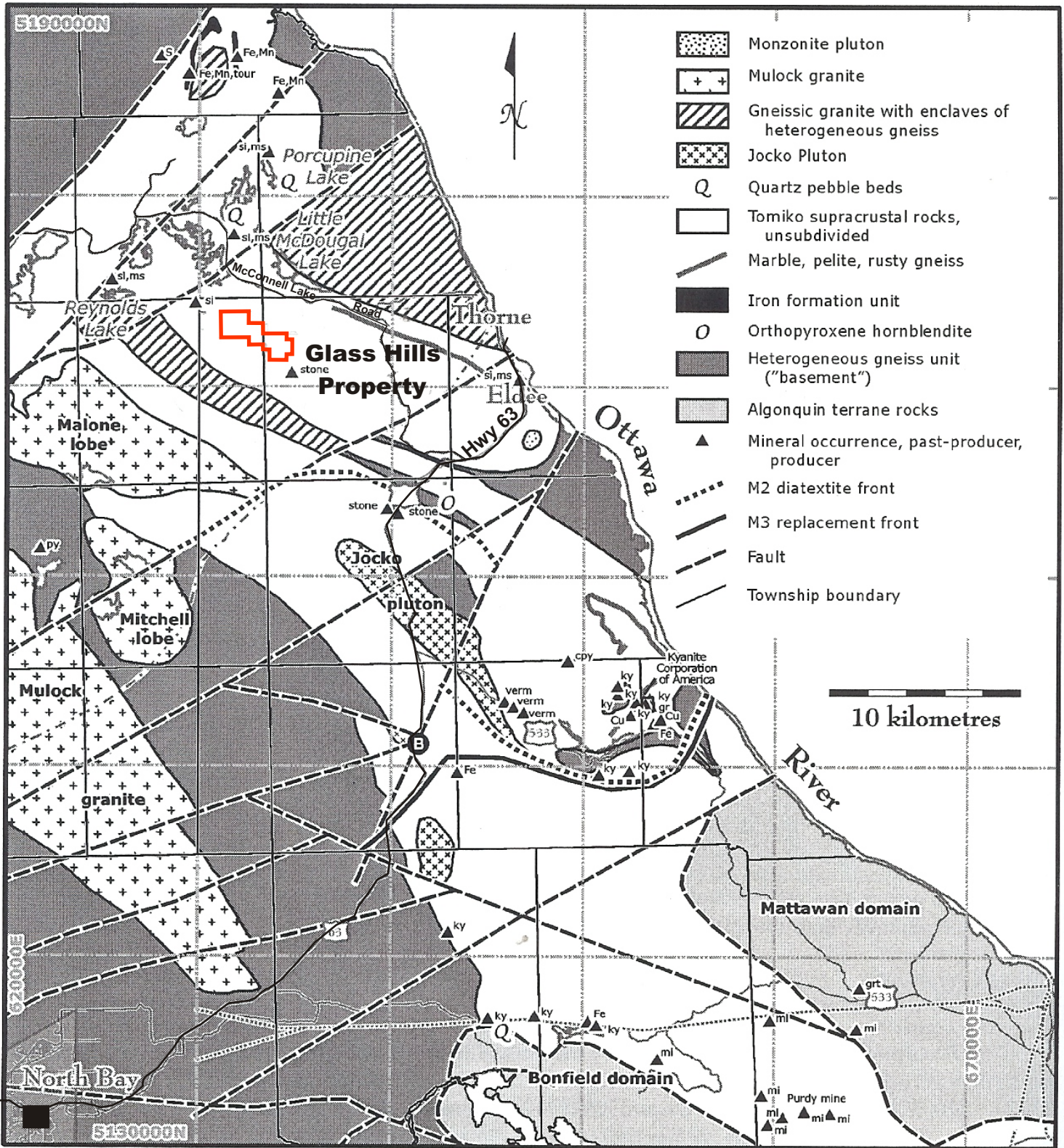
Figure 3. Location of the Glass Hills Property and the Regional Geology of the Tomiko Terrane
